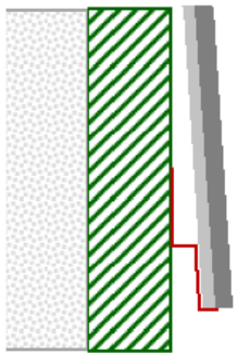
Starter Profile Trim (AL/ST60)
