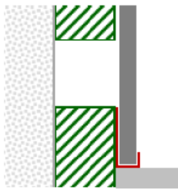
Connection Profile Trim (AL/755)
