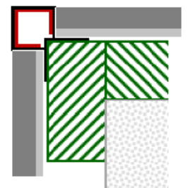
Corner Connection Trim (AL/125/CP)
