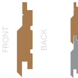
Ex 25mm x 100mm: NWSN1 SECRET FIX
