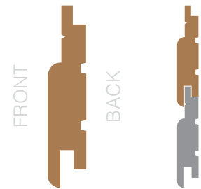
Ex 25mm x 100mm: NWSN3 SECRET FIX
