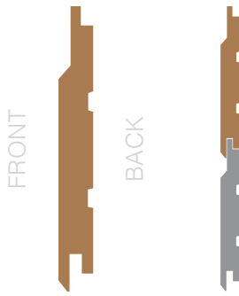
Ex 25mm x 150mm: NWC1 FACE FIX
